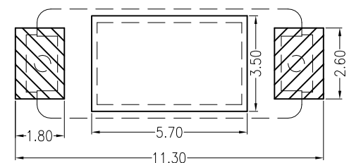
Board Layout General Tolerance: \pm 0.05
