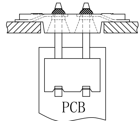
Assembly Layout
